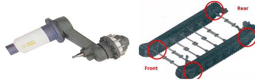
NSN 2530-01-0835438(9) NAME ARM & HUB ASSEMBLY, SUSPENSION
